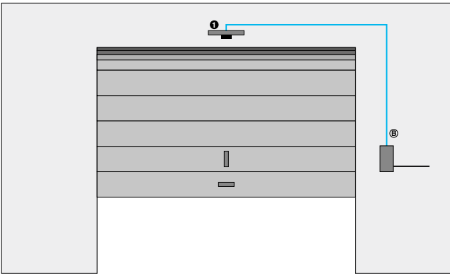
■ (B) Power cabling (230V) ■ 2x1,5 mm 2 +T cable
